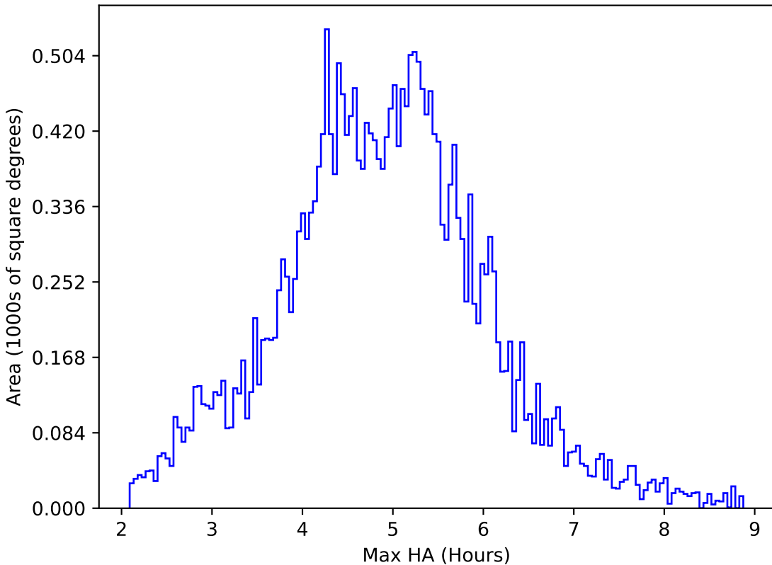
too_elab_r8_d2_gz_v3.4_10yrs All sky all bands: Max HA
