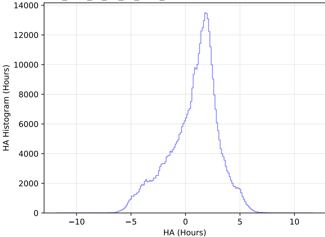
too_elab_r8_d2_gz_v3.4_10yrs WFD z band: HA Histogram
