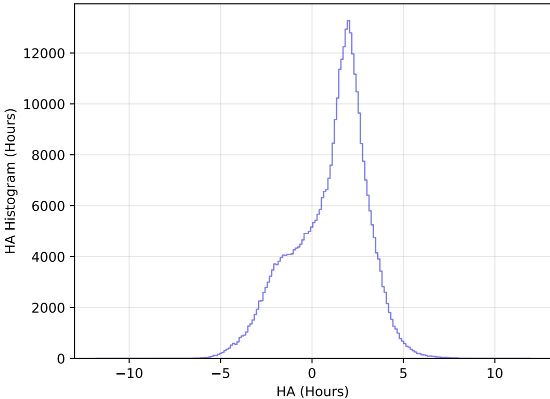
too_elab_r8_d2_gz_v3.4_10yrs WFD y band: HA Histogram
