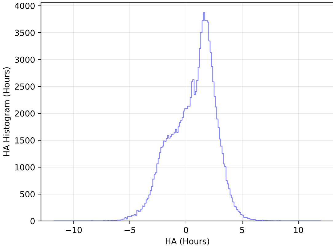
too_elab_r8_d2_gz_v3.4_10yrs WFD u band: HA Histogram
