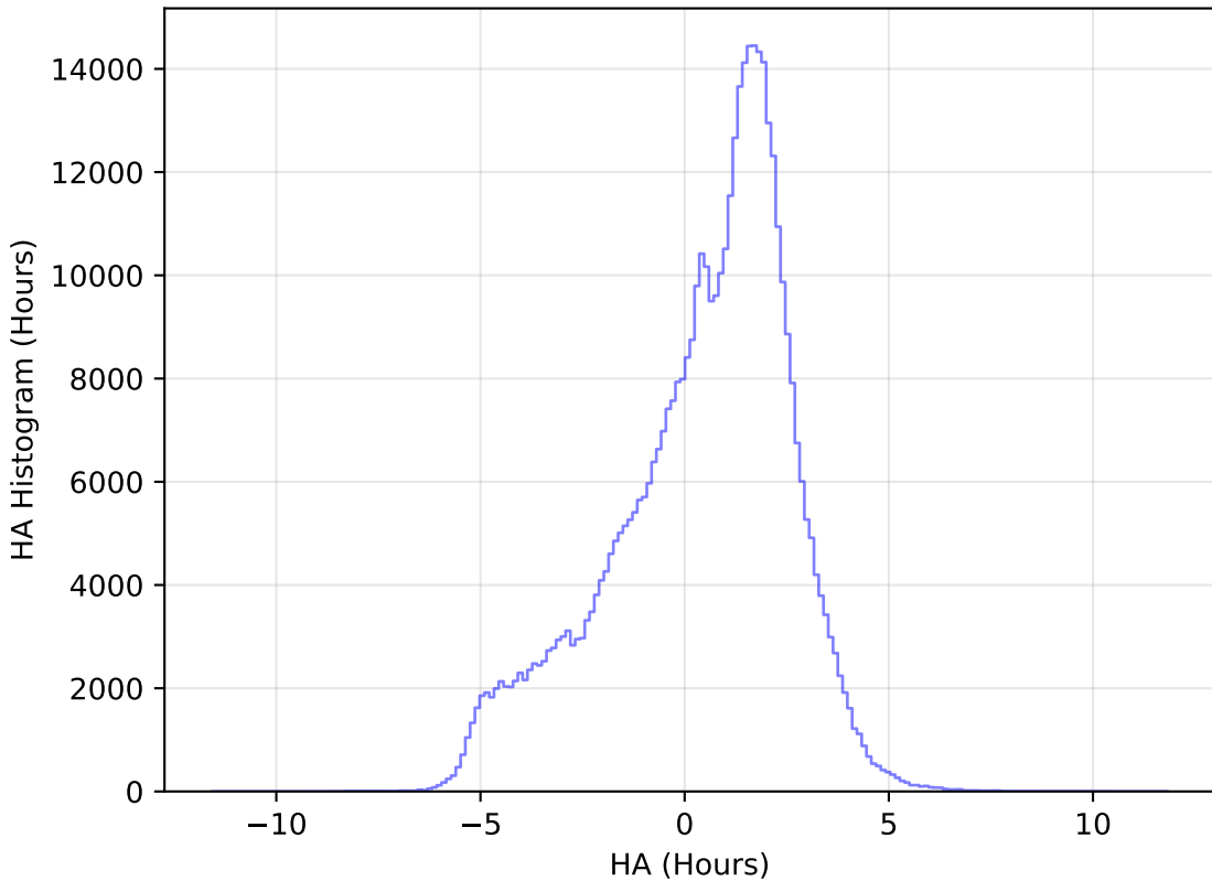
too_elab_r8_d2_gz_v3.4_10yrs WFD r band: HA Histogram
