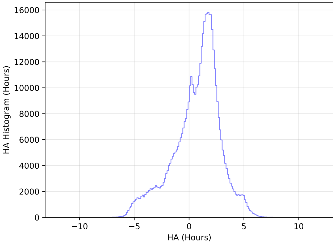
too_elab_r8_d2_gz_v3.4_10yrs WFD i band: HA Histogram
