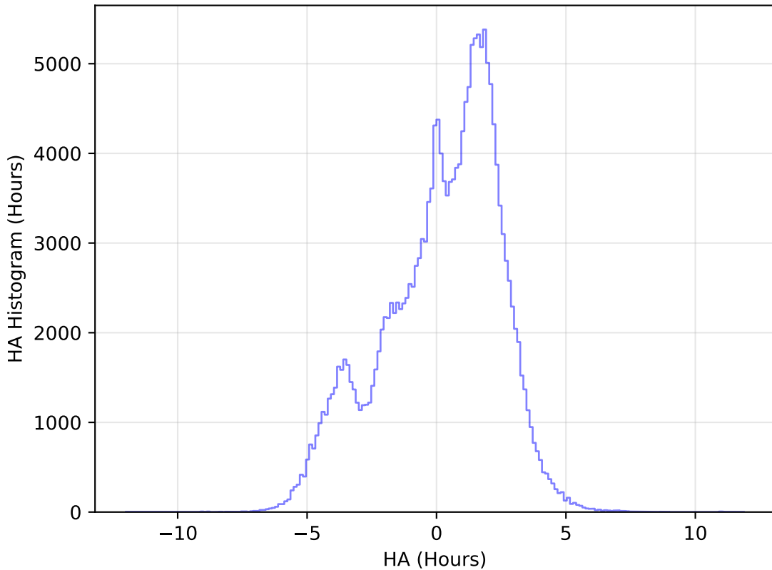
too_elab_r8_d2_gz_v3.4_10yrs WFD g band: HA Histogram
