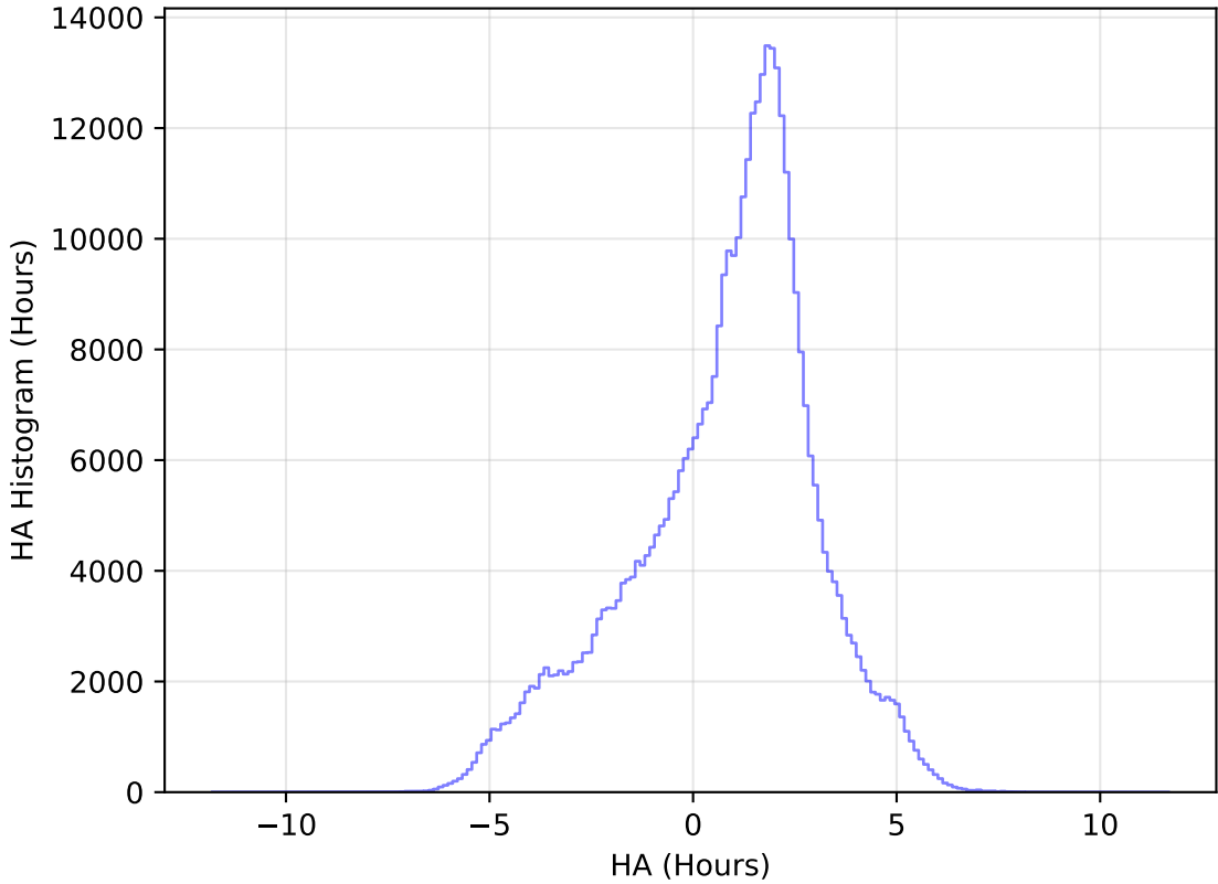
too_elab_r8_d2_gz_v3.4_10yrs All sky z band: HA Histogram
