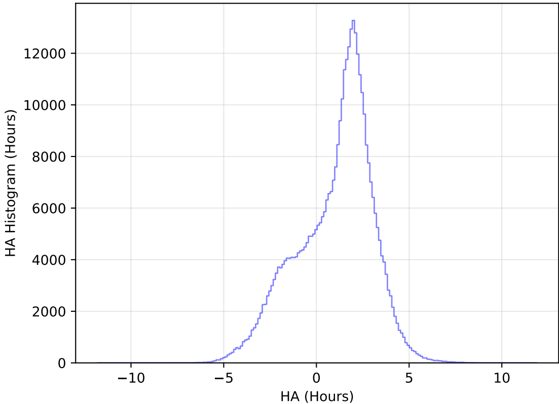
too_elab_r8_d2_gz_v3.4_10yrs All sky y band: HA Histogram
