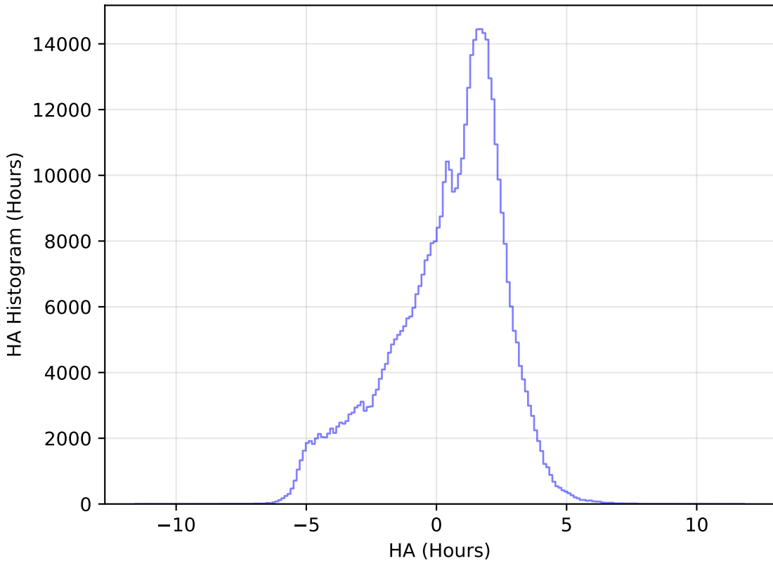
too_elab_r8_d2_gz_v3.4_10yrs All sky r band: HA Histogram
