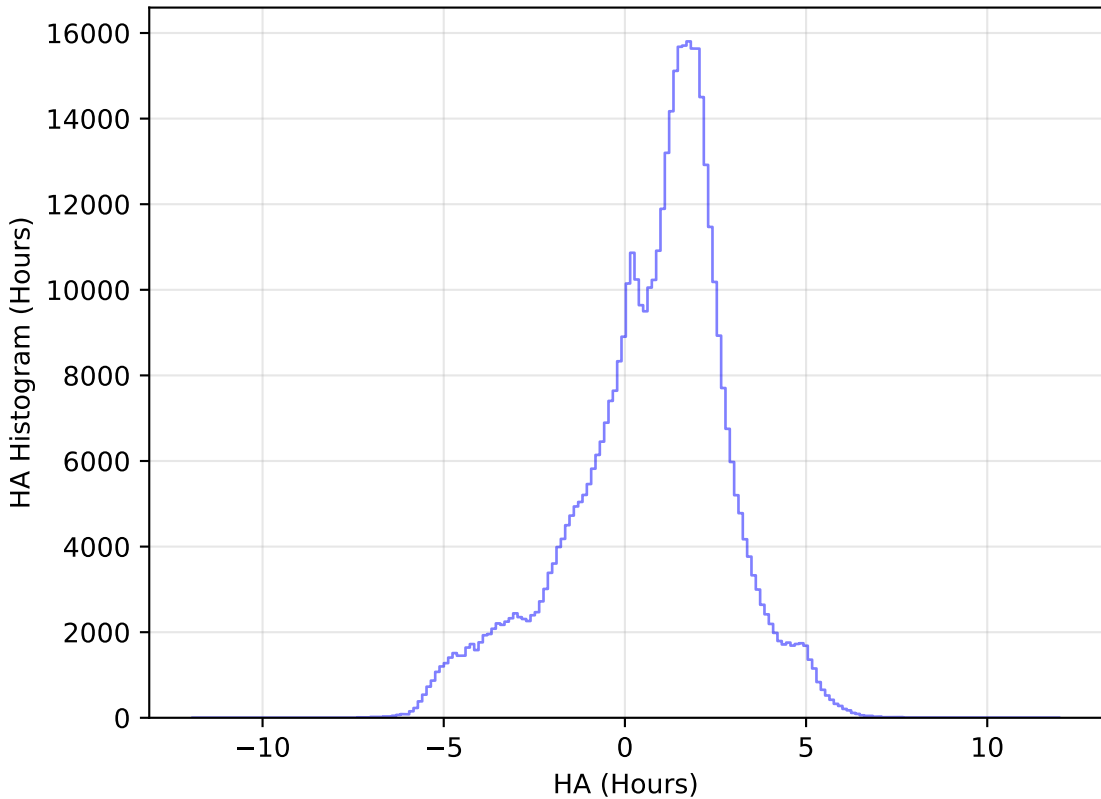
too_elab_r8_d2_gz_v3.4_10yrs All sky i band: HA Histogram
