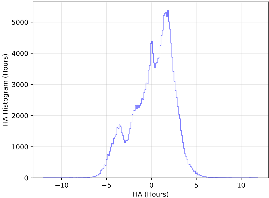
too_elab_r8_d2_gz_v3.4_10yrs All sky g band: HA Histogram
