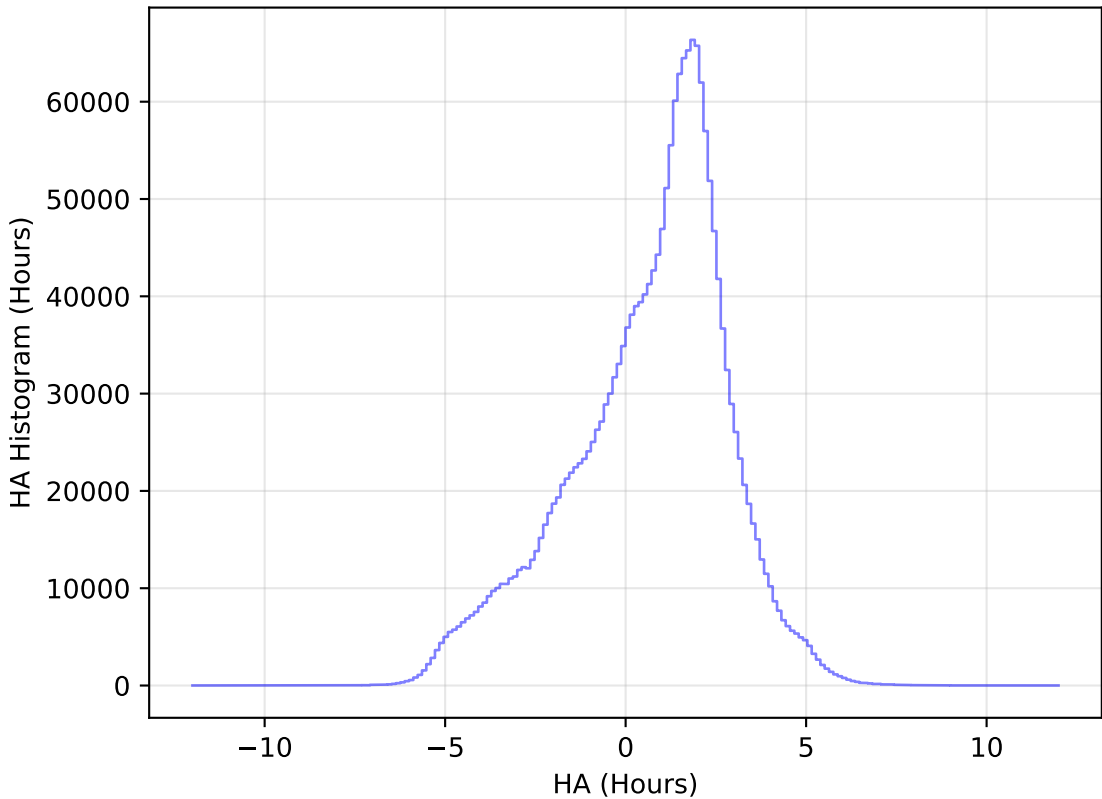
too_elab_r8_d2_gz_v3.4_10yrs All sky all bands: HA Histogram
