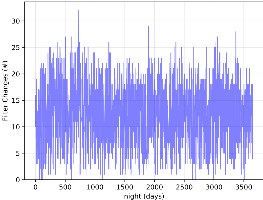
too_elab_r8_d2_gz_v3.4_10yrs Per Night: Filter Changes
