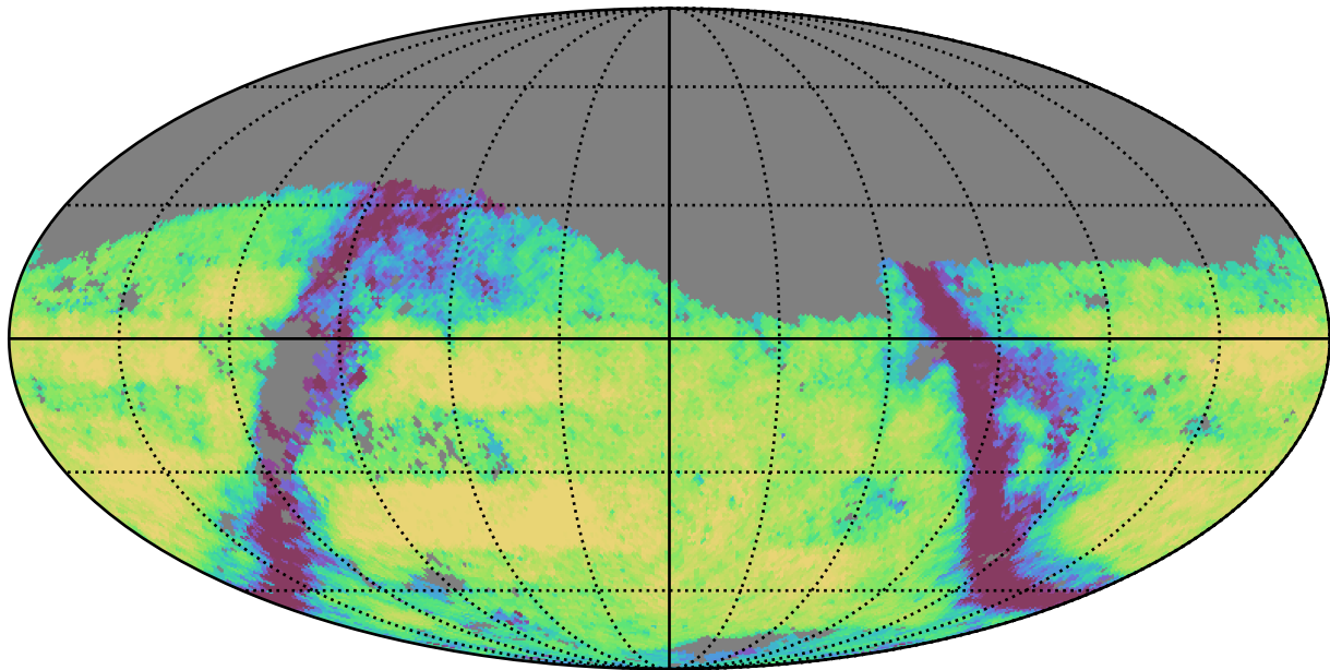
too_elab_r8_d2_gz_v3.4_10yrs Yr 3-4 g band: Exgal_CoaddM5
