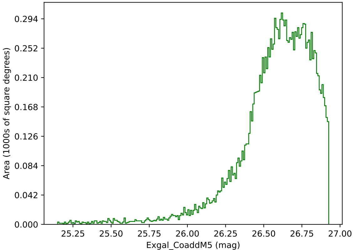
too_elab_r8_d2_gz_v3.4_10yrs WFD g band: Exgal_CoaddM5
