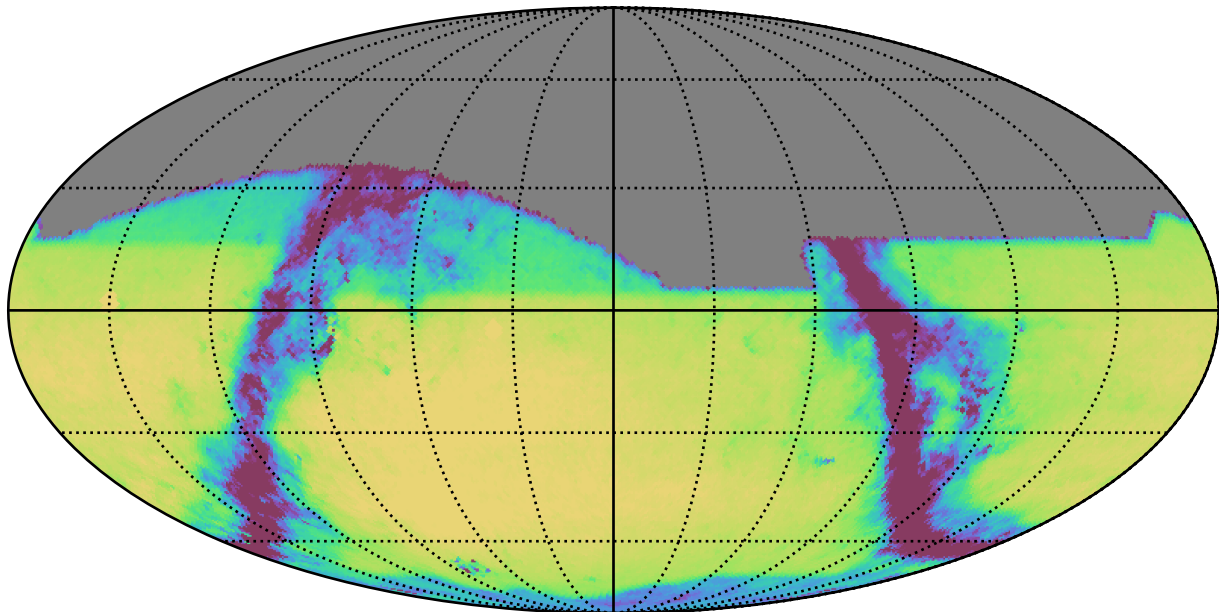
too_elab_r8_d2_gz_v3.4_10yrs All sky r band: Exgal_CoaddM5
