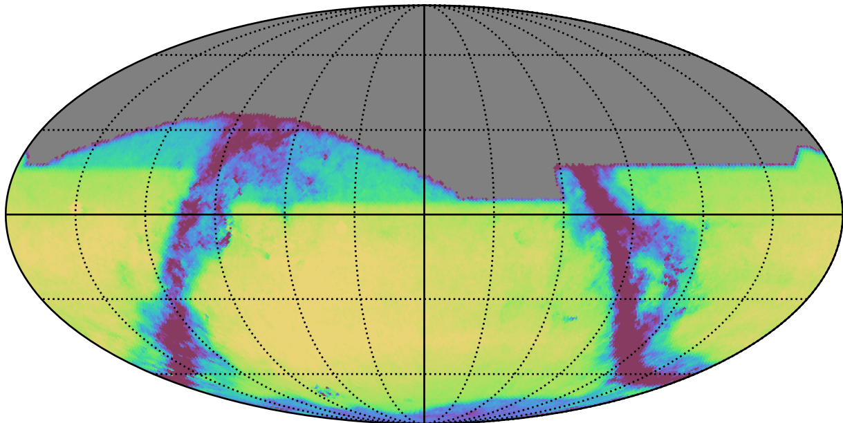
too_elab_r8_d2_gz_v3.4_10yrs All sky i band: Exgal_CoaddM5
