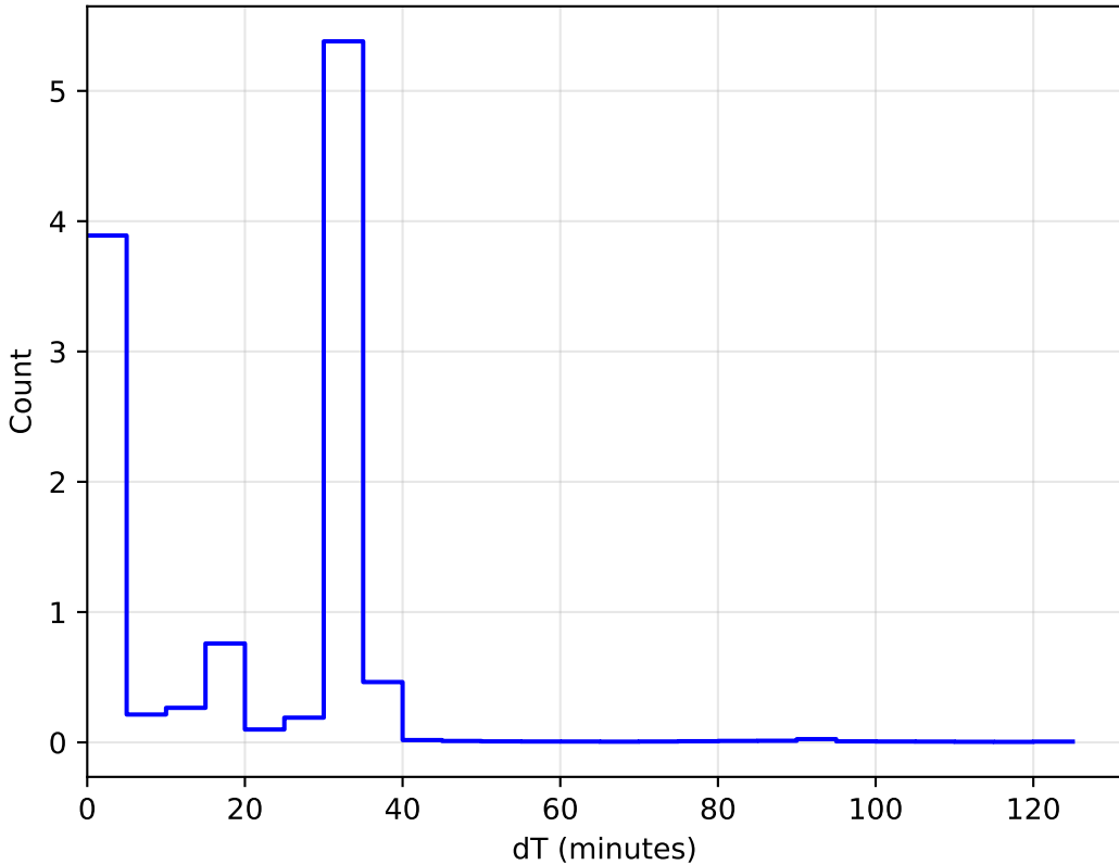
too_elab_r8_d2_gz_v3.4_10yrs WFD: DeltaT Histogram
