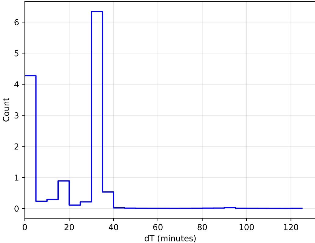
too_elab_r8_d2_gz_v3.4_10yrs All sky: DeltaT Histogram
