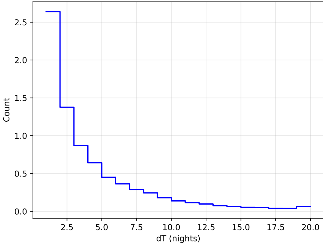
too_elab_r8_d2_gz_v3.4_10yrs WFD all bands: DeltaNight Histogram 1e6
