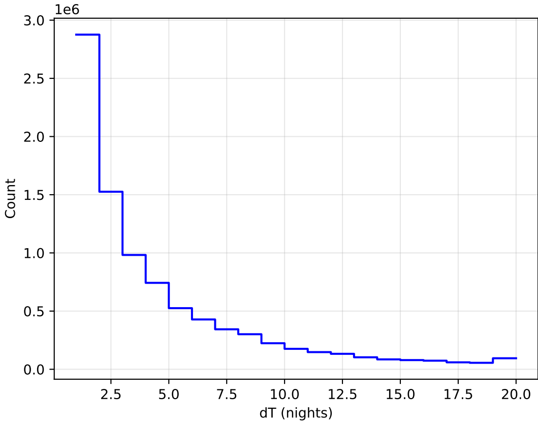
too_elab_r8_d2_gz_v3.4_10yrs All sky all bands: DeltaNight Histogram
