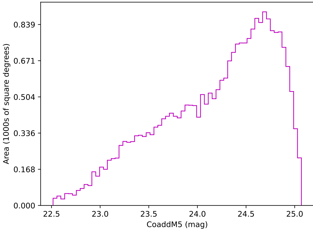
too_elab_r8_d2_gz_v3.4_10yrs Yr 3-4 z band: CoaddM5
