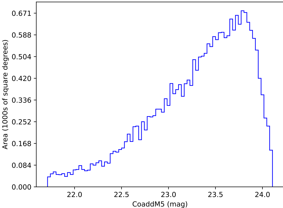
too_elab_r8_d2_gz_v3.4_10yrs Yr 3-4 y band: CoaddM5
