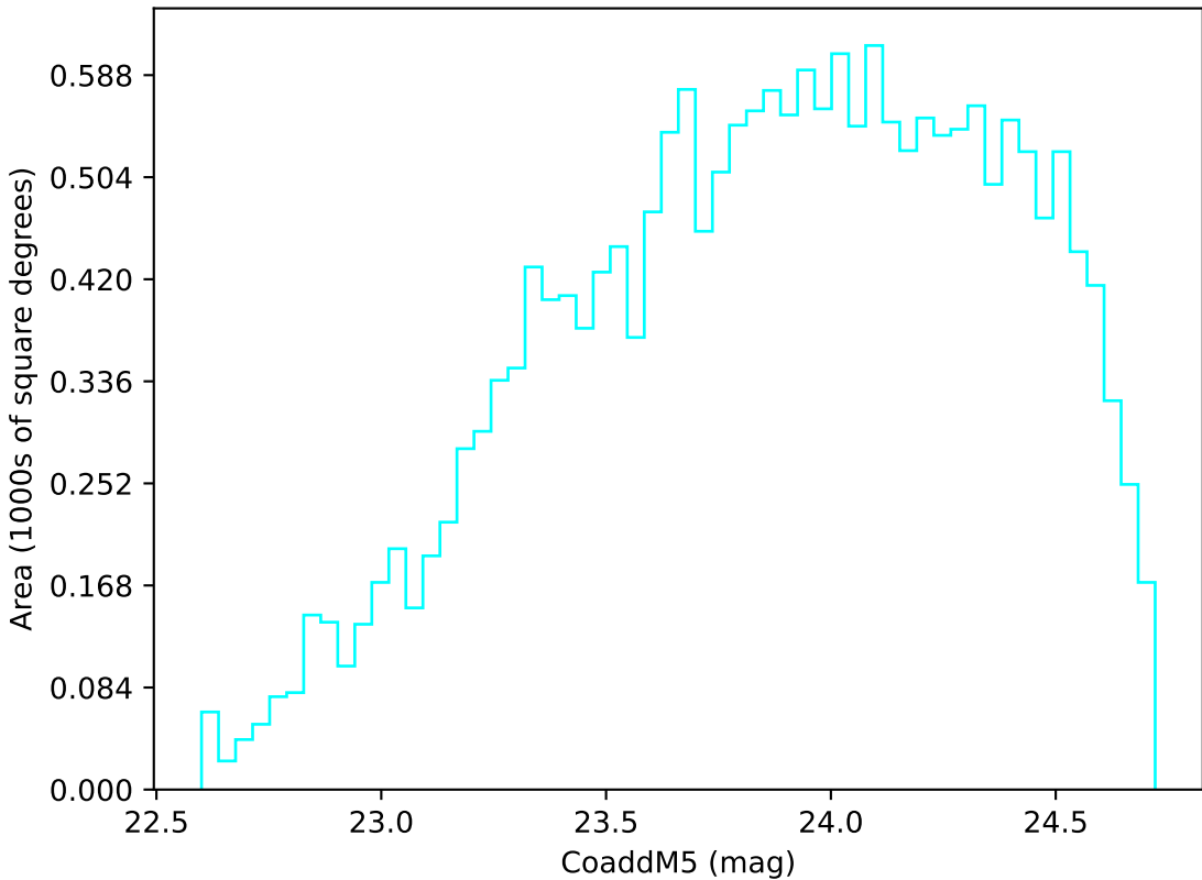
too_elab_r8_d2_gz_v3.4_10yrs Yr 3-4 u band: CoaddM5
