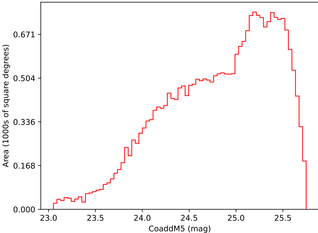
too_elab_r8_d2_gz_v3.4_10yrs Yr 3-4 i band: CoaddM5
