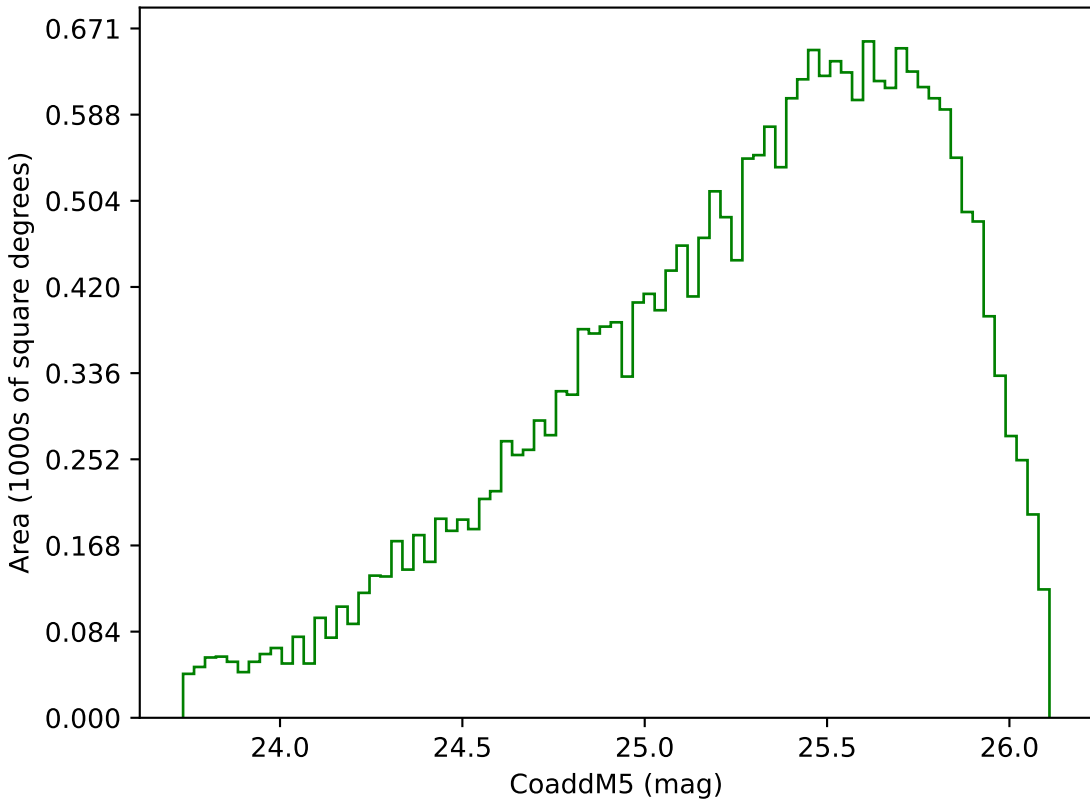
too_elab_r8_d2_gz_v3.4_10yrs Yr 3-4 g band: CoaddM5
