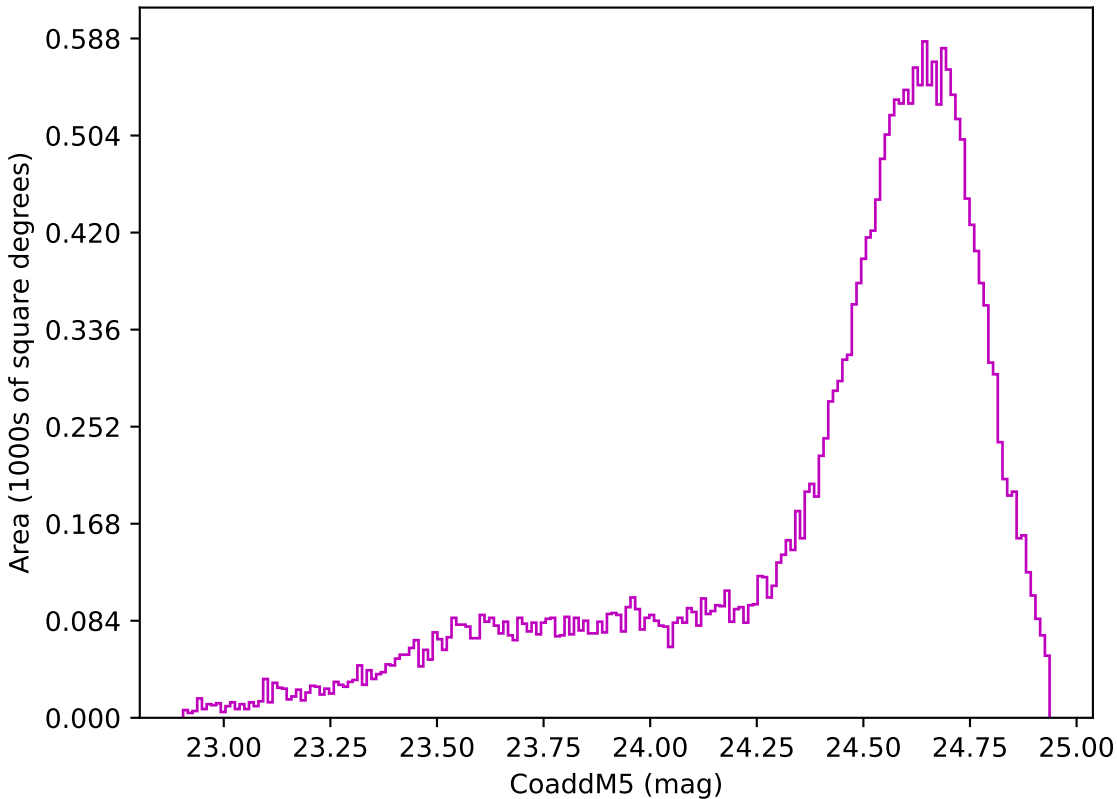
too_elab_r8_d2_gz_v3.4_10yrs Yr 1 z band: CoaddM5
