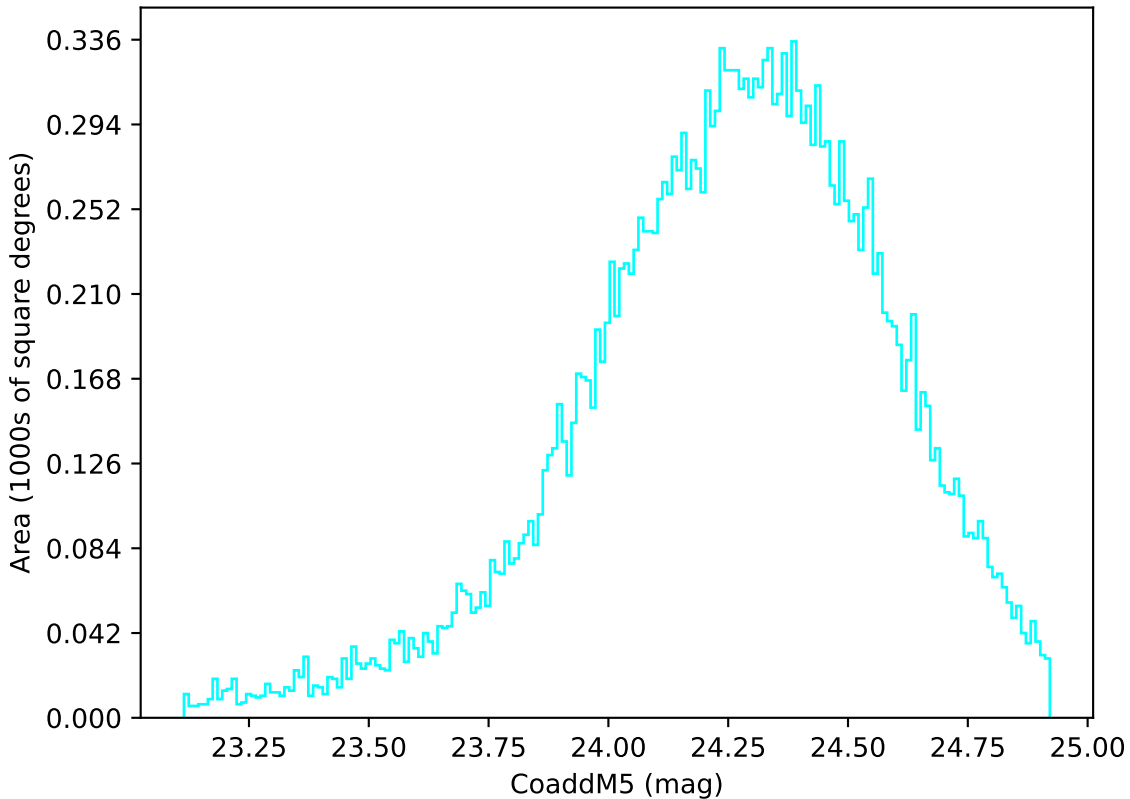
too_elab_r8_d2_gz_v3.4_10yrs Yr 1 u band: CoaddM5
