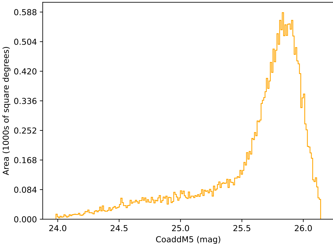
too_elab_r8_d2_gz_v3.4_10yrs Yr 1 r band: CoaddM5
