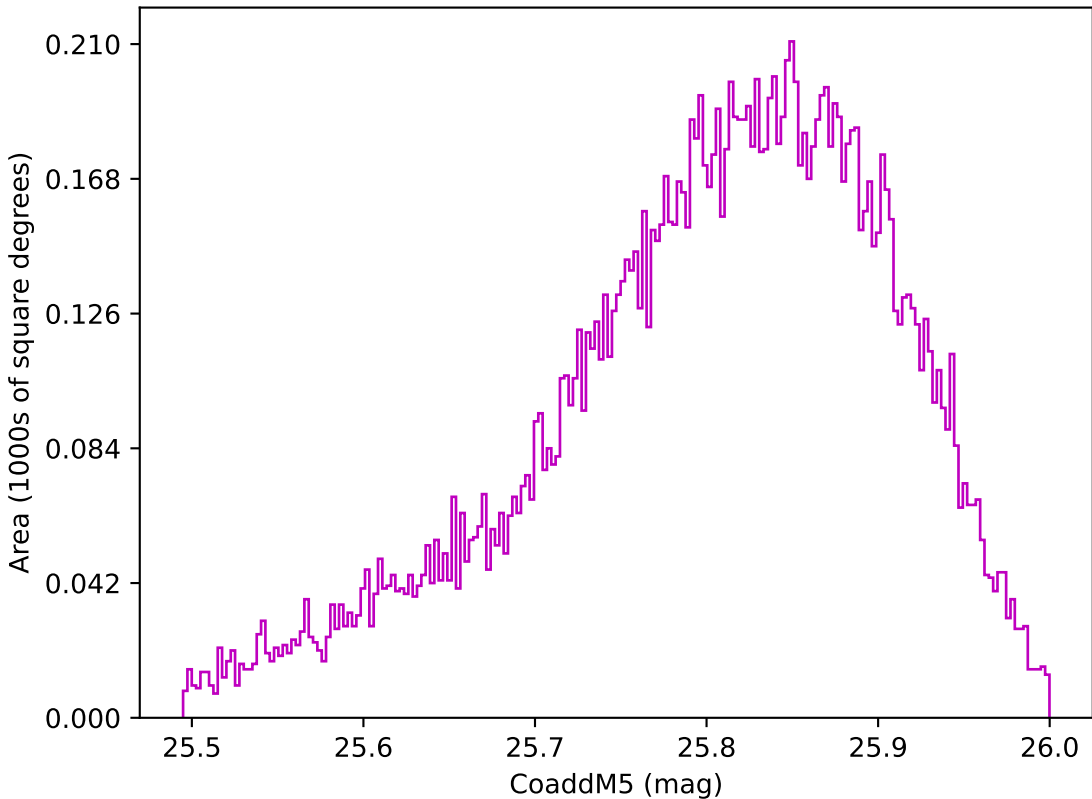
too_elab_r8_d2_gz_v3.4_10yrs WFD z band: CoaddM5
