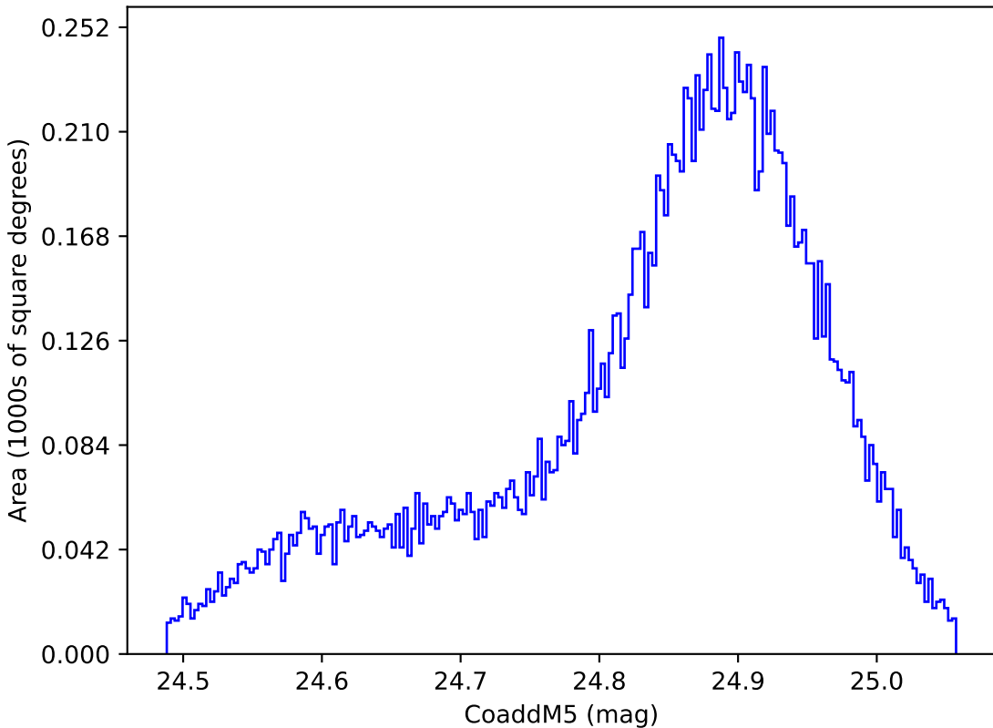
too_elab_r8_d2_gz_v3.4_10yrs WFD y band: CoaddM5
