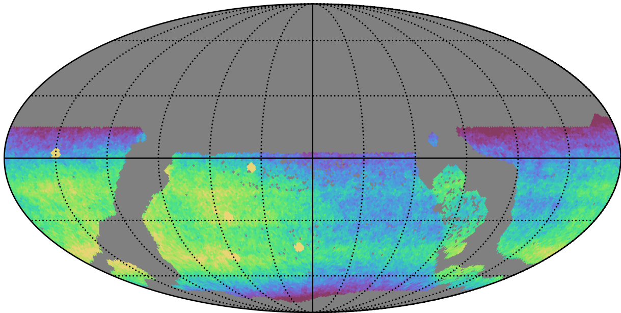
too_elab_r8_d2_gz_v3.4_10yrs WFD r band: CoaddM5
