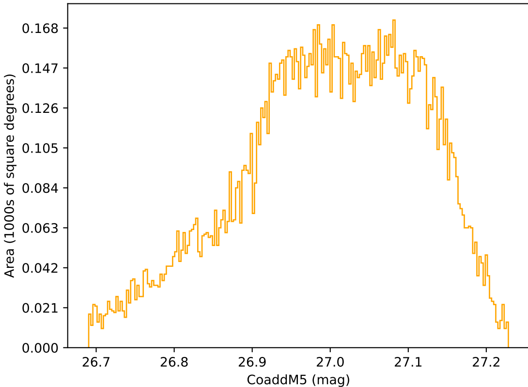
too_elab_r8_d2_gz_v3.4_10yrs WFD r band: CoaddM5
