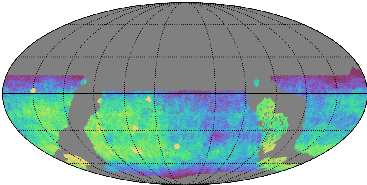
too_elab_r8_d2_gz_v3.4_10yrs WFD g band: CoaddM5
