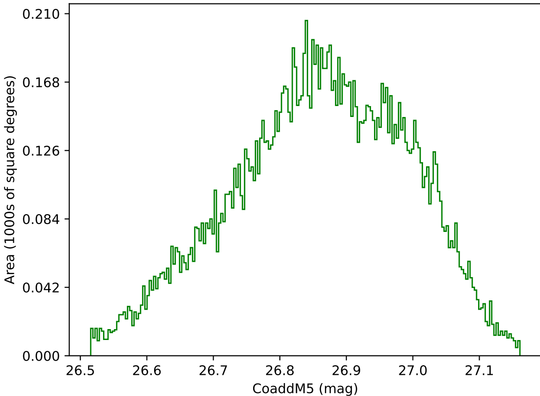
too_elab_r8_d2_gz_v3.4_10yrs WFD g band: CoaddM5
