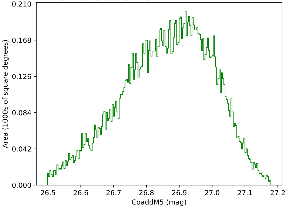
too_elab_r8_d2_gz_v3.4_10yrs WFD g band: CoaddM5
