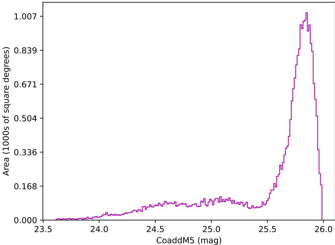
too_elab_r8_d2_gz_v3.4_10yrs All sky z band: CoaddM5
