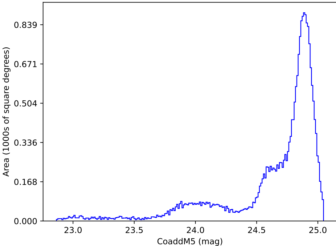
too_elab_r8_d2_gz_v3.4_10yrs All sky y band: CoaddM5
