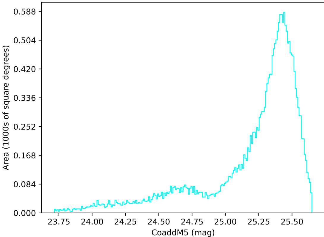
too_elab_r8_d2_gz_v3.4_10yrs All sky u band: CoaddM5
