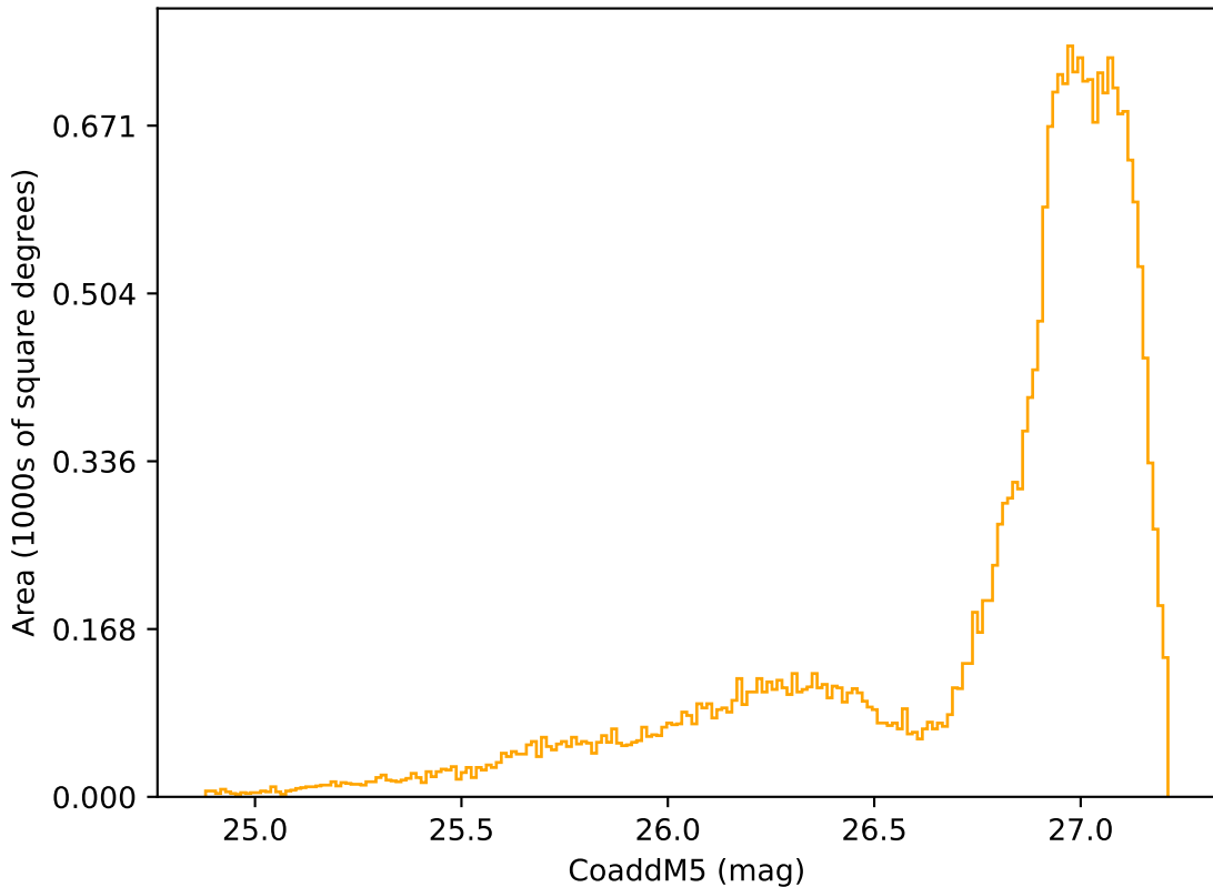
too_elab_r8_d2_gz_v3.4_10yrs All sky r band: CoaddM5
