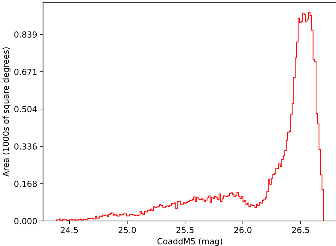
too_elab_r8_d2_gz_v3.4_10yrs All sky i band: CoaddM5
