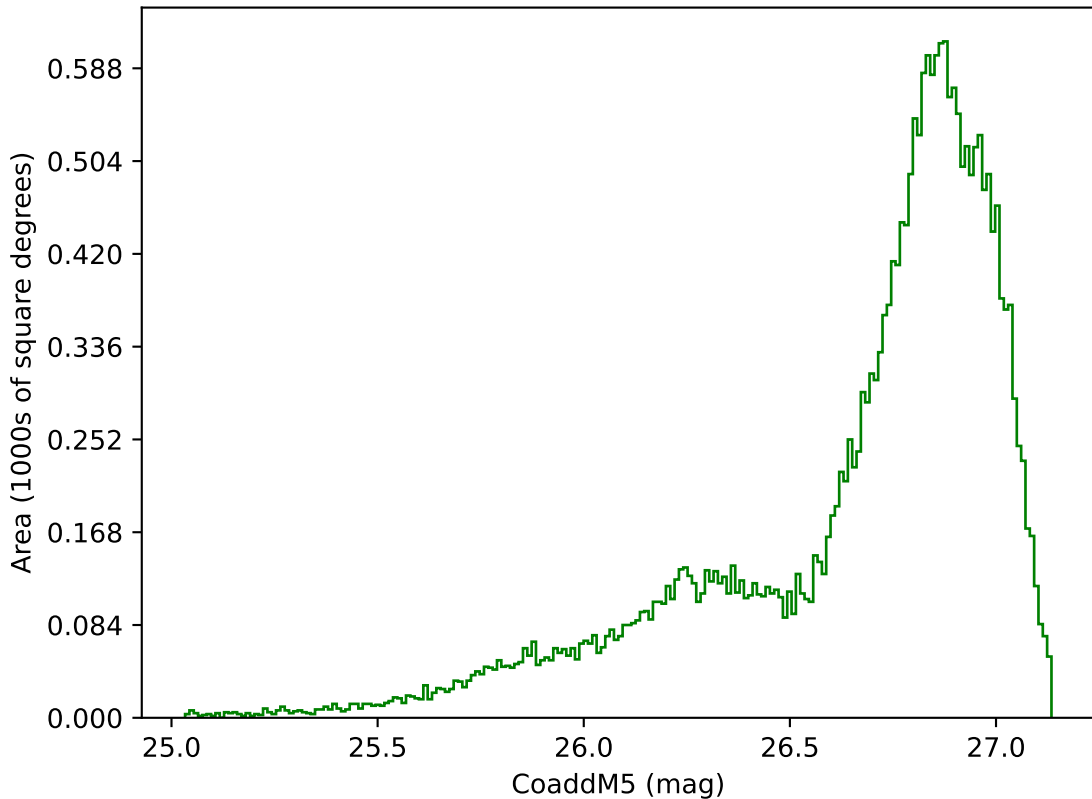
too_elab_r8_d2_gz_v3.4_10yrs All sky g band: CoaddM5
