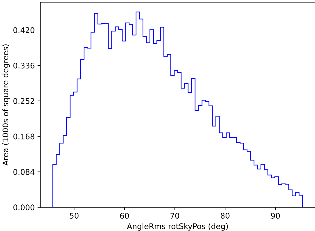
too_elab_r8_d2_gz_v3.4_10yrs WFD u band: AngleRms rotSkyPos
