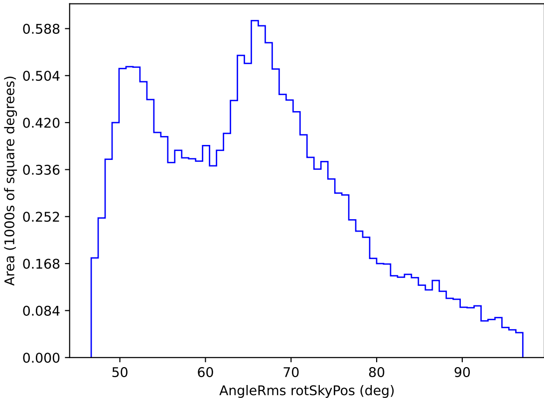
too_elab_r8_d2_gz_v3.4_10yrs WFD r band: AngleRms rotSkyPos
