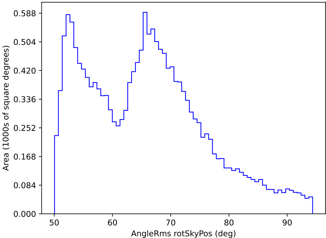
too_elab_r8_d2_gz_v3.4_10yrs WFD all bands: AngleRms rotSkyPos
