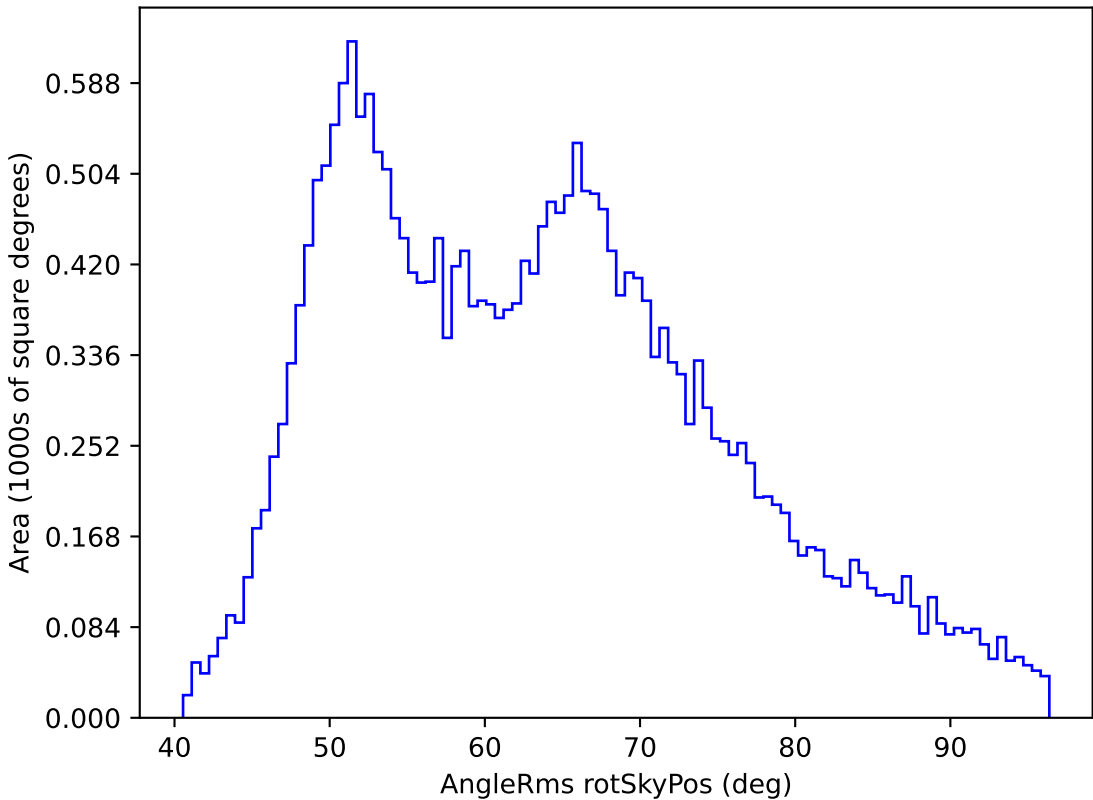
too_elab_r8_d2_gz_v3.4_10yrs All sky r band: AngleRms rotSkyPos
