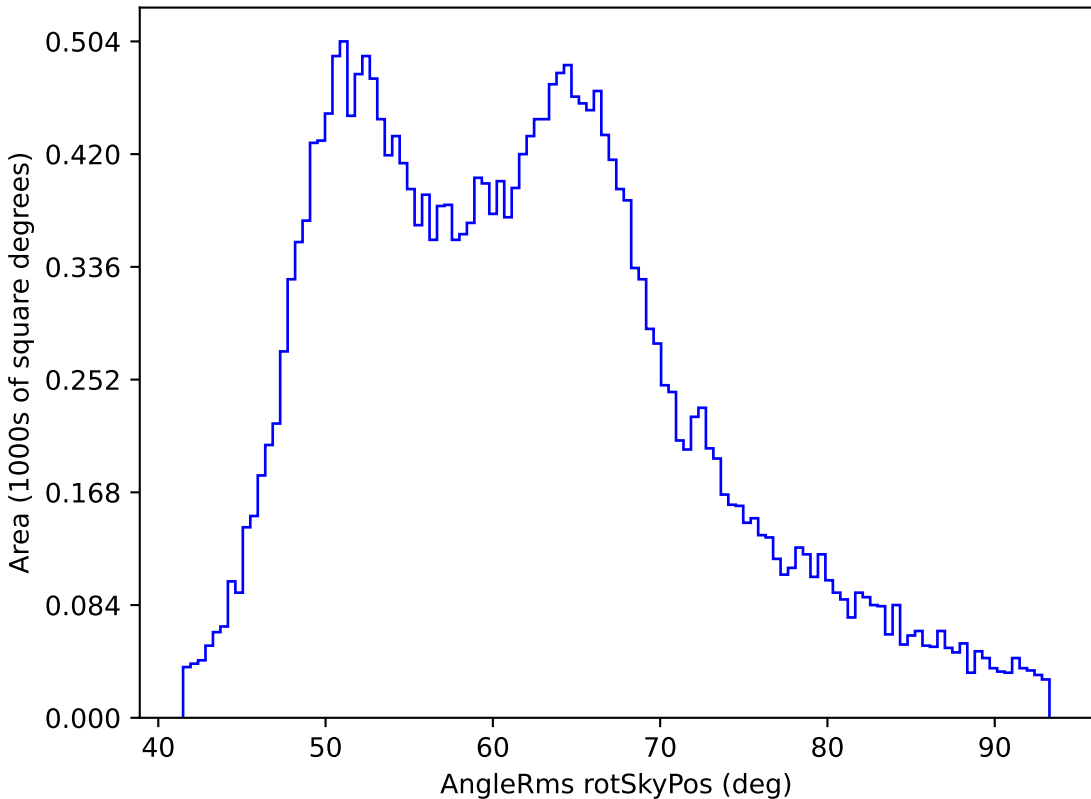
too_elab_r8_d2_gz_v3.4_10yrs All sky i band: AngleRms rotSkyPos
