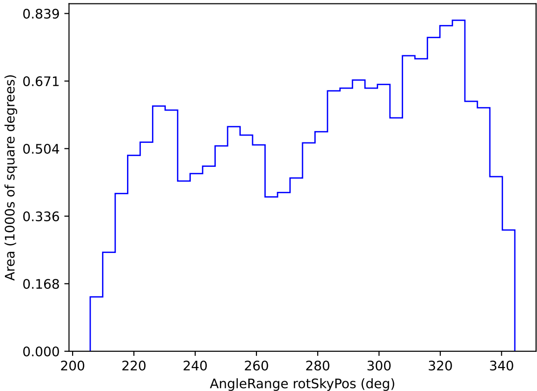
too_elab_r8_d2_gz_v3.4_10yrs WFD r band: AngleRange rotSkyPos
