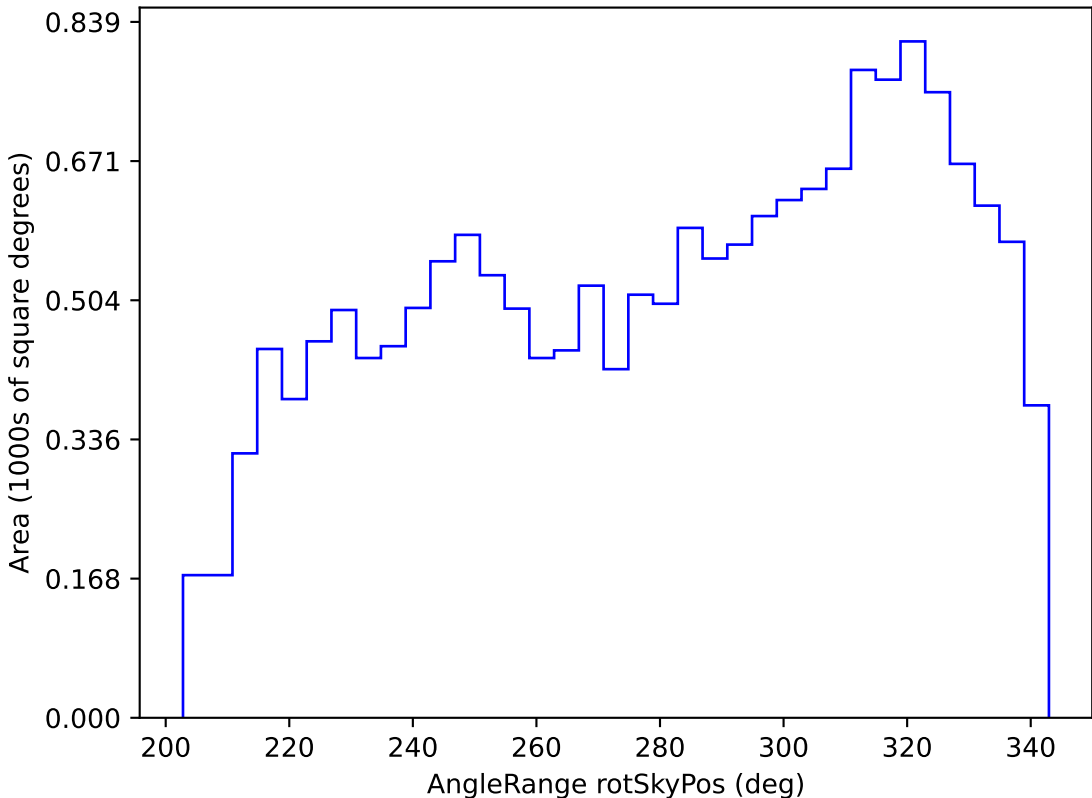
too_elab_r8_d2_gz_v3.4_10yrs WFD i band: AngleRange rotSkyPos
