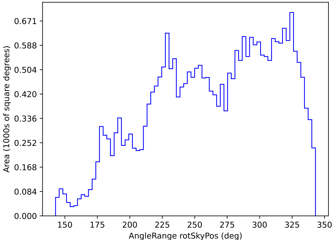
too_elab_r8_d2_gz_v3.4_10yrs All sky r band: AngleRange rotSkyPos
